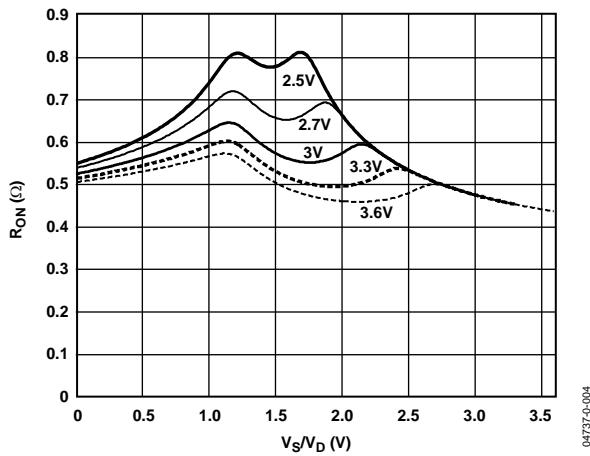
Figure 4. On-Resistance vs. V_D/V_S , V_{DD} = 2.5V to 3.6V
