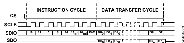
Figure 10. Serial Register Interface Timing LSB First
