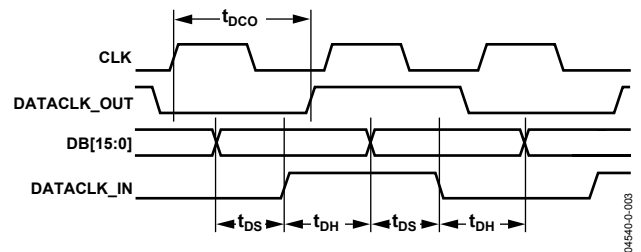
Figure 3. Double Datarate (DDR) Mode
