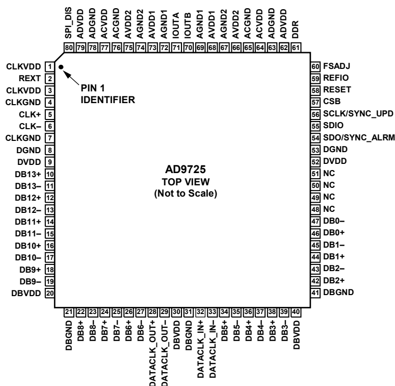
Figure 4. Pin Configuration
