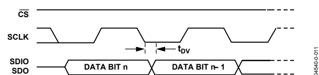
Figure 12. Timing Diagram for Register READ to AD9725
