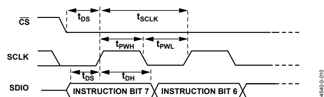
Figure 11. Timing Diagram for Register Write to AD9725
