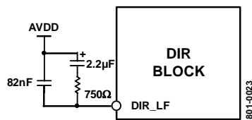
Figure 22. DIR loop Filter Components
