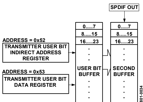
Figure 32. Transmitter User Bit Buffer
