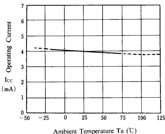
Operating Current vs. Temperature ( V^+/V^-=\pm 15\text{V} )
