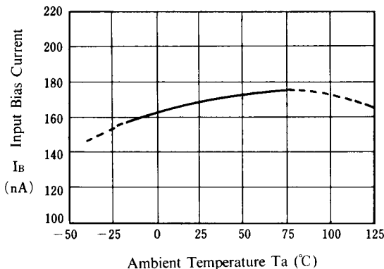
Input Bias Current vs. Temperature ( V^+/V^-=\pm 15\text{V} )
