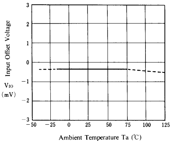
Input Offset Voltage vs. Temperature ( V^+/V^-=\pm 15\text{V} )
