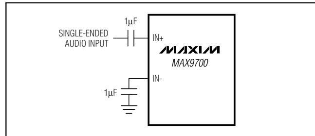
Figure 6. Single-Ended Input
