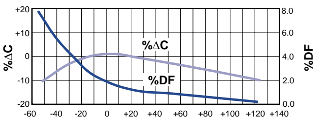
Figure 4. Temperature °C Capacitance & DF vs Temperature - X7R
