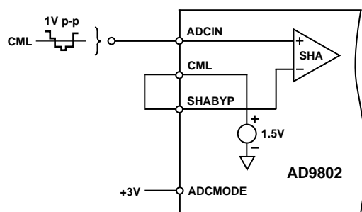
Figure 22. DC-Coupled Input
