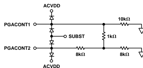
Figure 7. Pin 29 (PGACONT1) and Pin 30 (PGACONT2)
