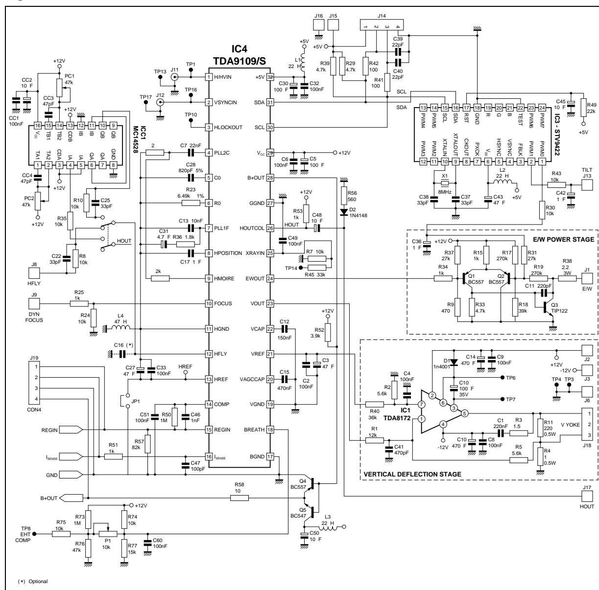
Figure 39 : Demonstration Board
