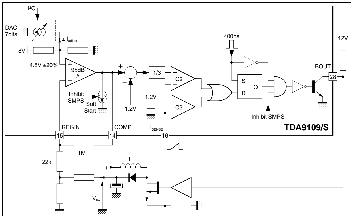
Figure 17 : DC/DC Converter
