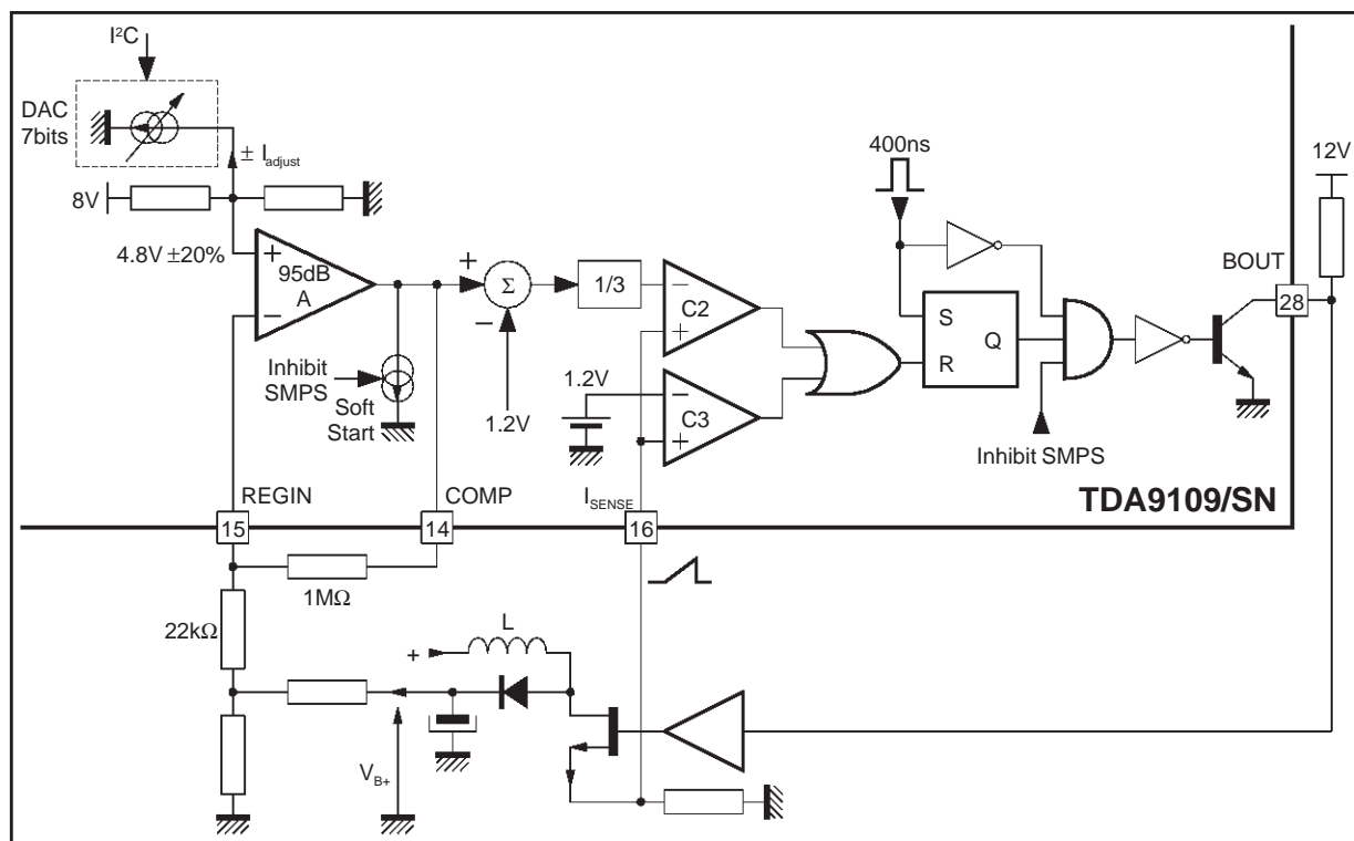
Figure 17 : DC/DC Converter
