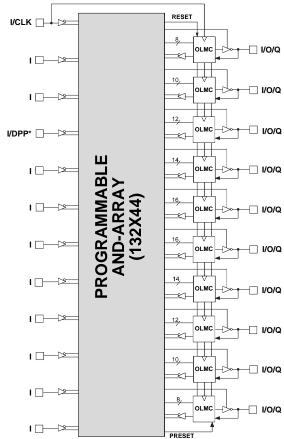
*GAL22LV10ZD Only
