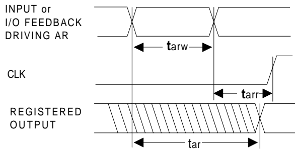
Asynchronous Reset
