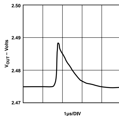
Figure 19. Major-Code Transition
