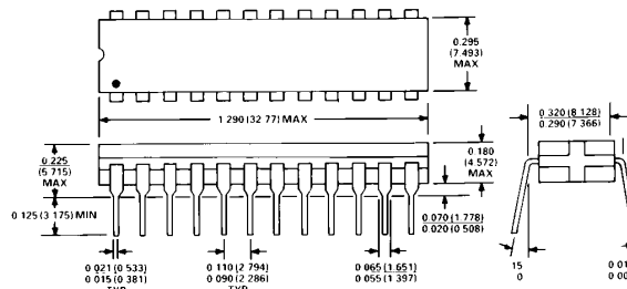
24-Pin Cerdip (Q-24) 1
