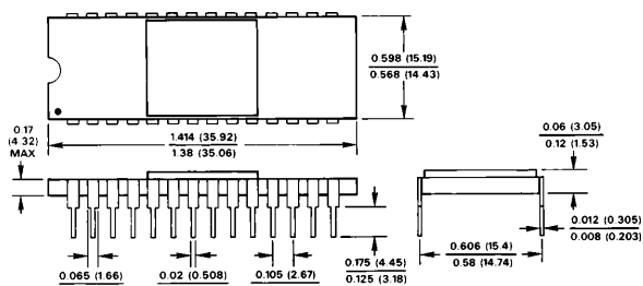
28-Pin Ceramic DIP (D-28) 1
