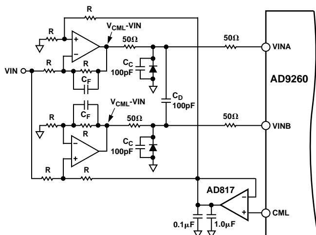
Figure 57. DC-Coupled Differential Driver with Level-Shifting
