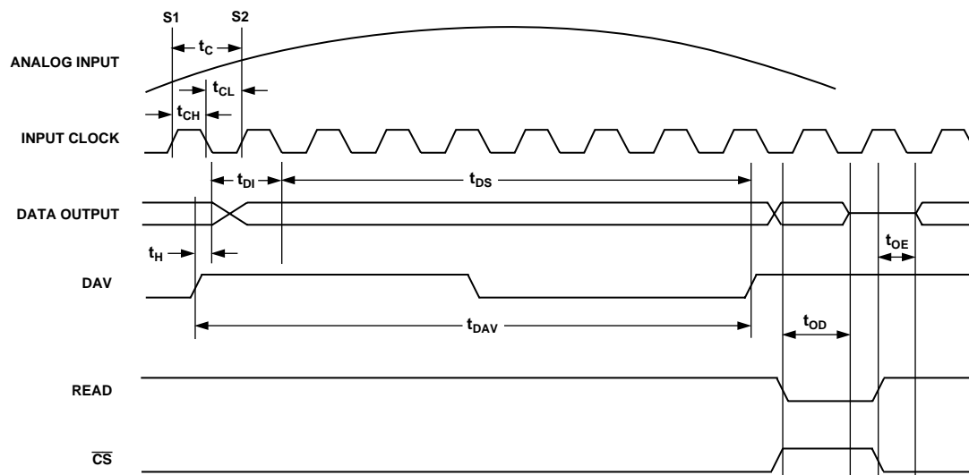
Figure 4. Timing Diagram
