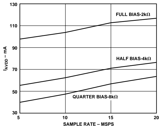
Figure 64. I_{AVDD} vs. Sample Rate ( AVDD = +5 V, Mode 1×–4×)
