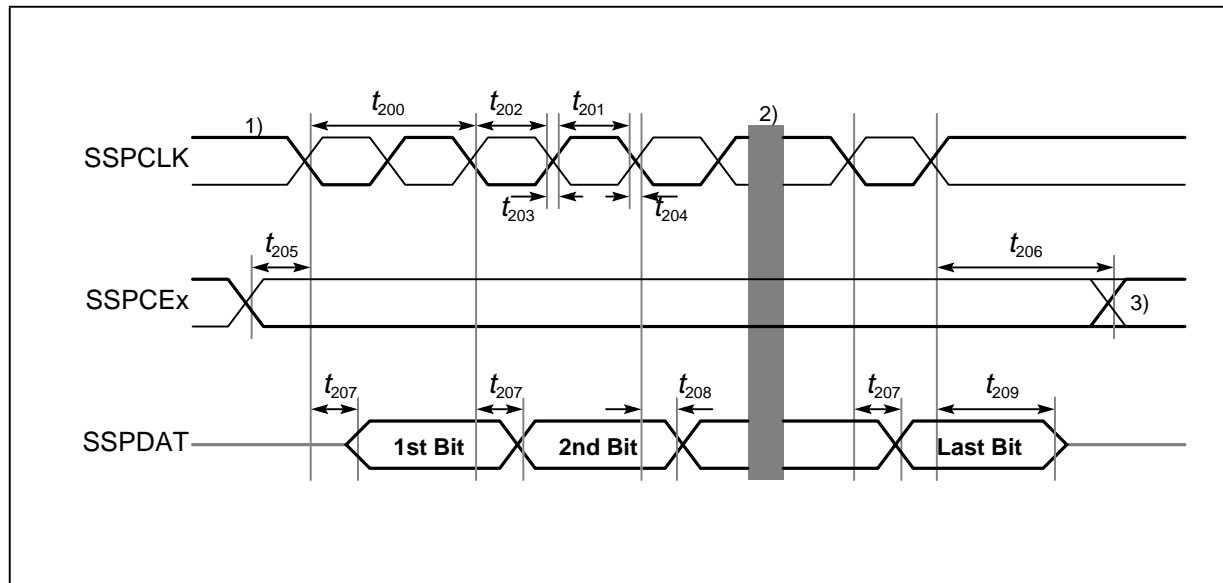
Figure 25 SSP write timing
