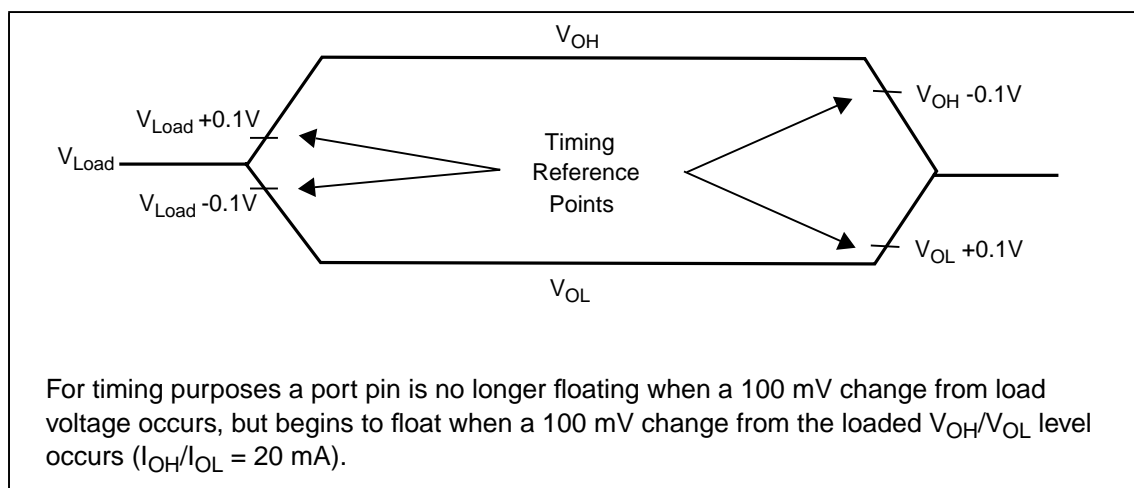
Figure 10 Float waveforms
