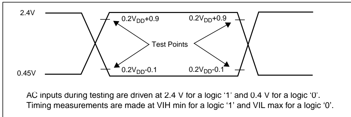
Figure 9 Input/output waveforms
