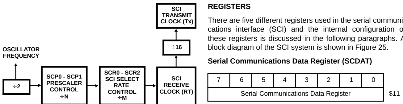
FIGURE 26. RATE GENERATOR DIVISION
