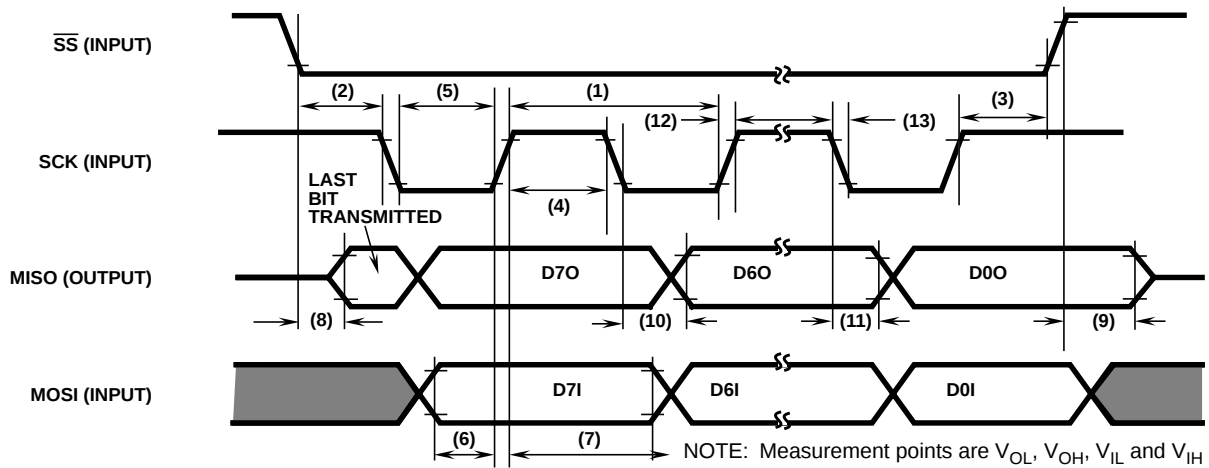
FIGURE 3F. SPI SLAVE TIMING CPOL = 1, CPHA = 1
