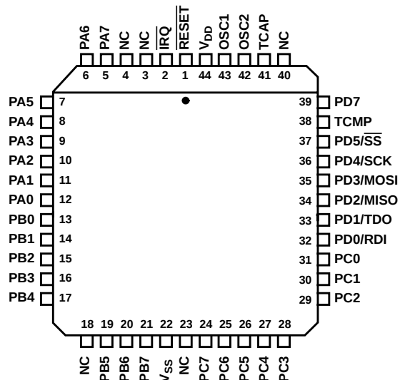
N SUFFIX (PLCC) TOP VIEW
