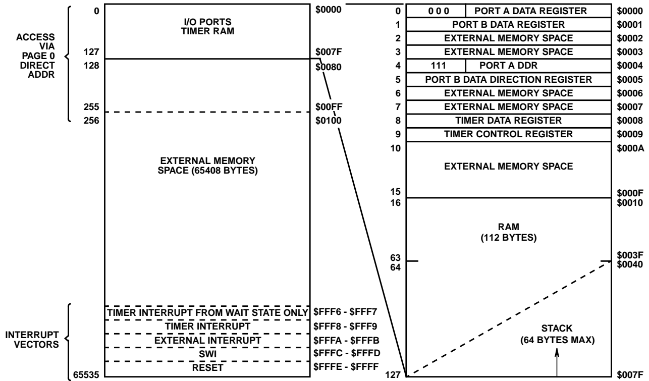
FIGURE 12B. CDP6805E3 ADDRESS MAP
