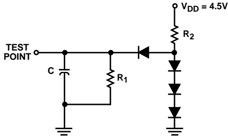
TTL EQUIVALENT
