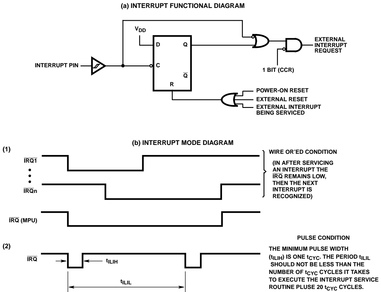
FIGURE 16. EXTERNAL INTERRUPT
