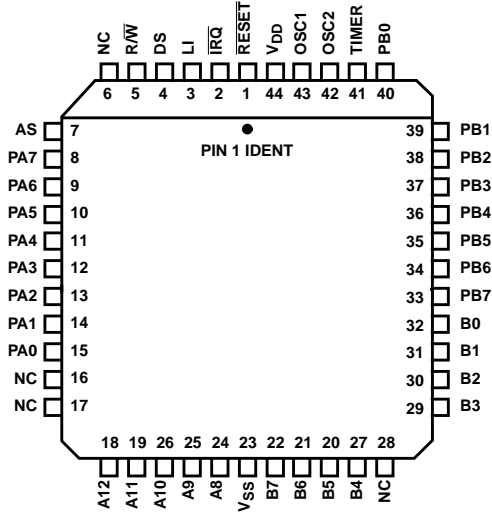
CDP6805E2 (PLCC) TOP VIEW
