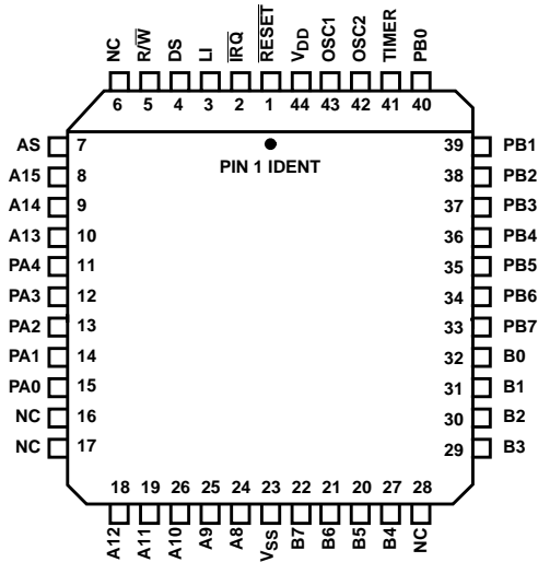
CDP6805E3 (PLCC) TOP VIEW
