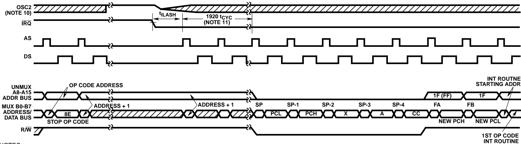
FIGURE 8. INTERRUPT RECOVERY FROM STOP INSTRUCTION TIMING WAVEFORMS
