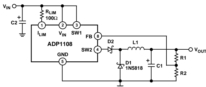
Figure 17. Step-Down Model, V_{OUT} > 6.2 V
