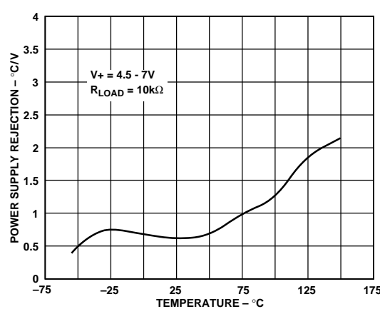
Figure 20. Power Supply Rejection vs. Temperature
