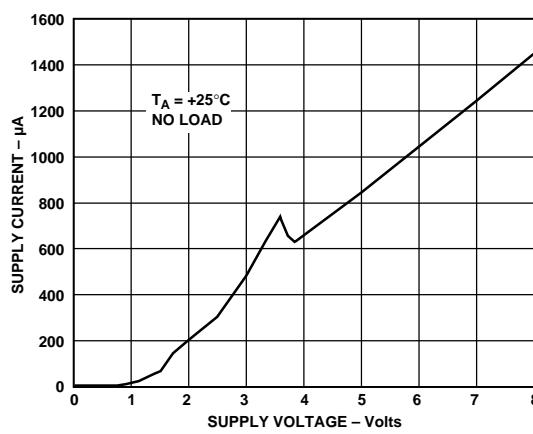
Figure 19. Supply Current vs. Supply Voltage
