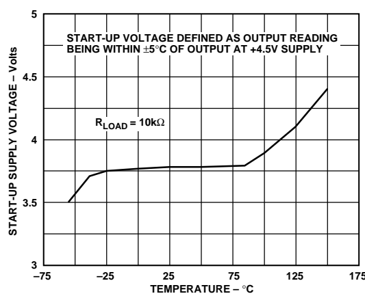
Figure 18. Start-Up Voltage vs. Temperature
