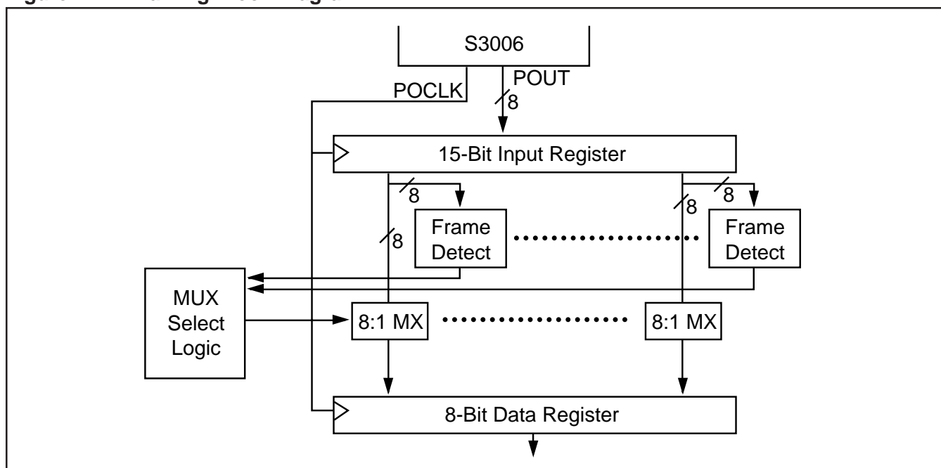
Figure 1. E4 Framing Block Diagram
