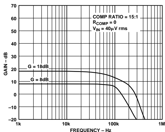
Figure 6. GBW Curves vs. VCA Gain
