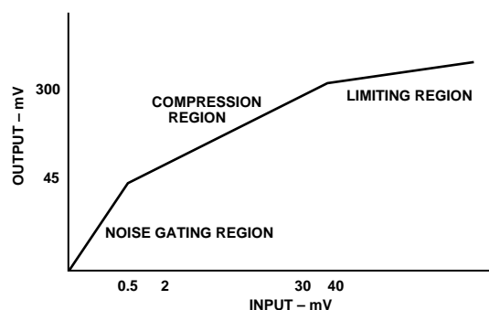
Figure 18. Transfer Characteristic
