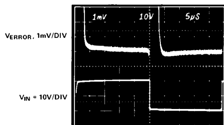
Figure 26. Settling Characteristic Detail—AD544
