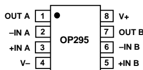
8-Lead Narrow-Body SO (S Suffix)
