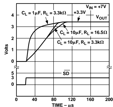
Figure 16. Turn On
