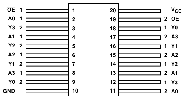
HCTS244KTR (FLATPACK), CDFF4-F20 TOP VIEW
