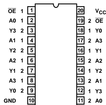
HCTS244DTR (SBDIP), CDIP2-T20 TOP VIEW
