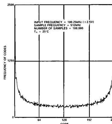
Figure 10. AD7821 Histogram Plot
