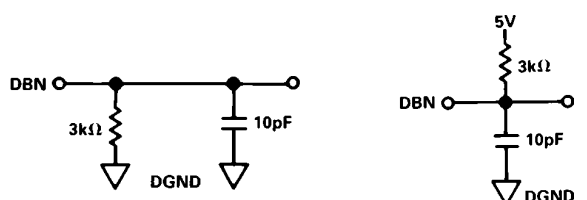
Figure 1. Load Circuits for Data Access Time Test
