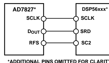
Figure 18. Interfacing to the DSP56xxx
