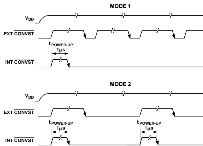
Figure 8. Power-Up Times
