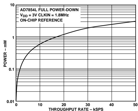
Figure 27. Power vs. Throughput AD7854L
