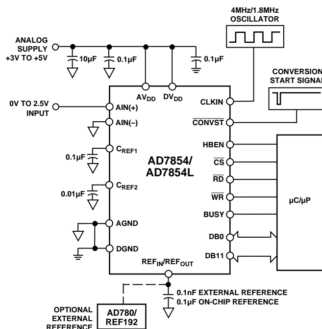
Figure 8. Typical Circuit
