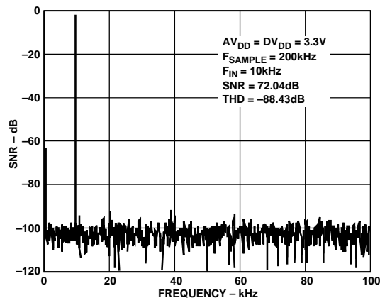
Figure 18. FFT Plot
