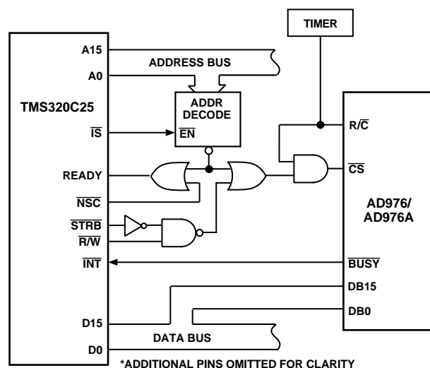
Figure 20. AD976/AD976A to TMS320C25 Interface
