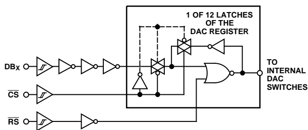
Figure 4. Digital Control Logic
