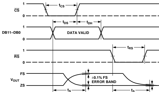
Figure 3. Timing Diagram
