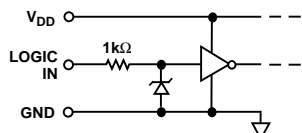
Figure 28. Equivalent Digital Input ESD Protection
