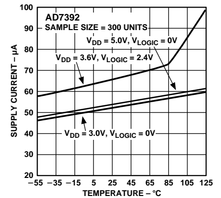
Figure 13. Supply Current vs. Temperature
