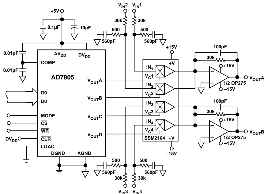
Figure 44. Low Cost, Two-Channel Mixer
