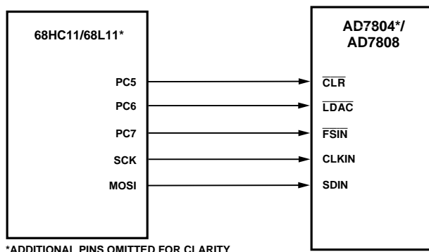
Figure 36. AD7804/AD7808-68HC11/68L11 Interface
