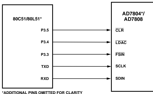
Figure 37. AD7804/AD7808-80C51/80L51 Interface
