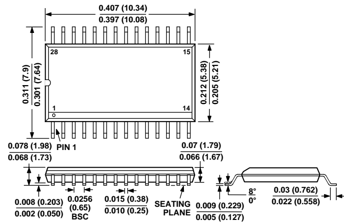
RS-28 28-Lead Shrink Small Outline Package (SSOP)
