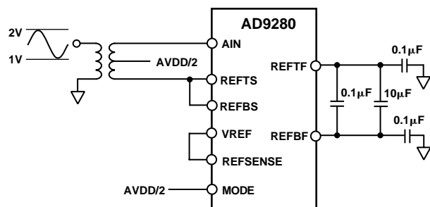
Figure 29. Differential Input
