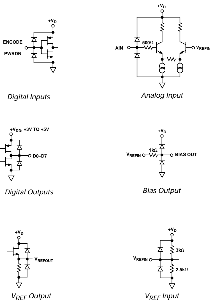
Figure 18. Equivalent Circuits
