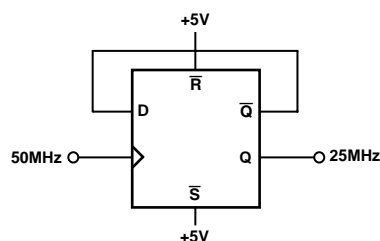
Figure 33. Divide-by-Two Clock Circuit
