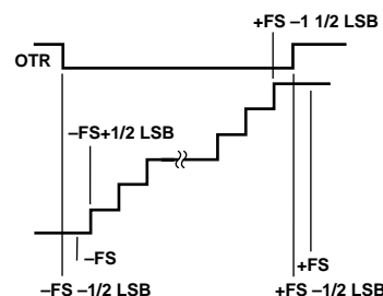
Figure 31. Output Data Format
