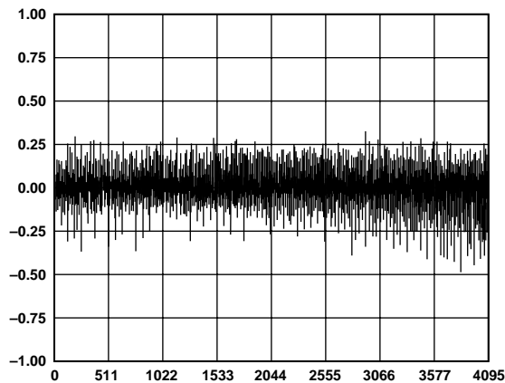
Figure 2. Typical DNL
