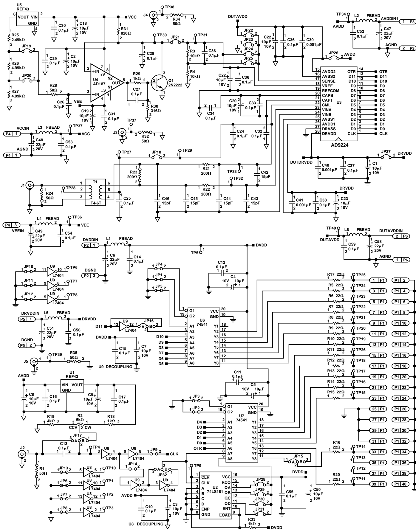
Figure 44. Evaluation Board Schematic
