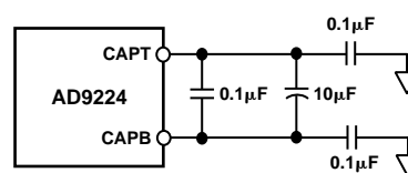
Figure 17. Recommended CAPT/CAPB Decoupling Network
