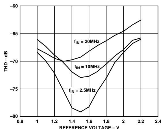
Figure 26b. THD vs. Reference Voltage
