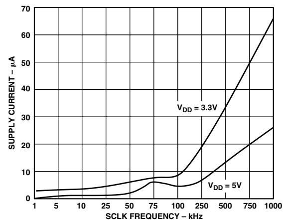
Figure 7. Standby Supply Current vs. SCLK Frequency
