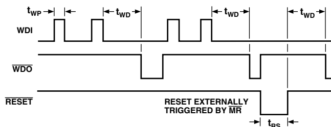
Figure 4. Watchdog Timing
