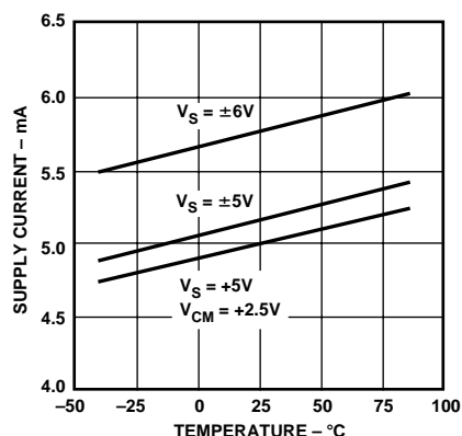
Figure 10. Supply Current vs. Temperature
