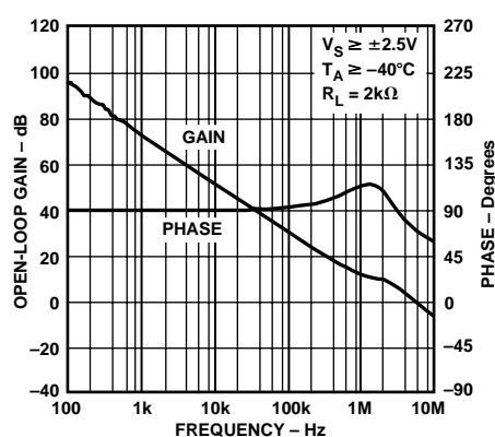
Figure 9. Open-Loop Gain and Phase vs. Frequency
