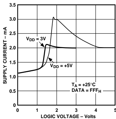
Figure 6. Supply Current vs. Logic Input Voltage
