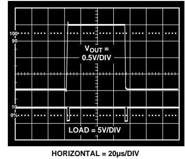
Figure 11. Large Signal Settling Time
