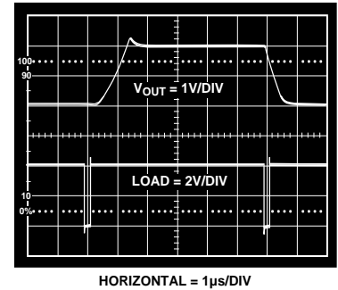
Figure 10. Detail Settling Time
