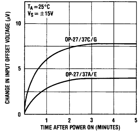
Warm-Up Drift
