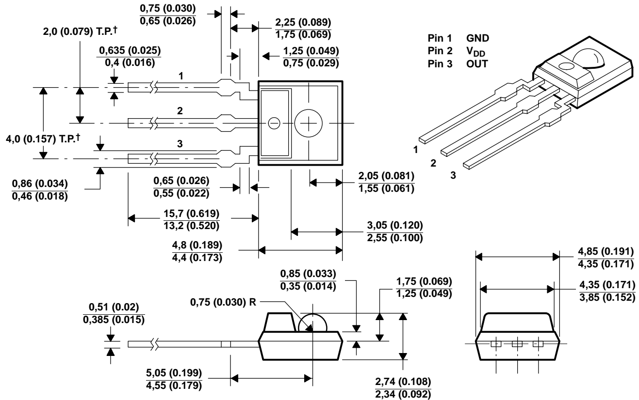
Figure 7. Mechanical Data
