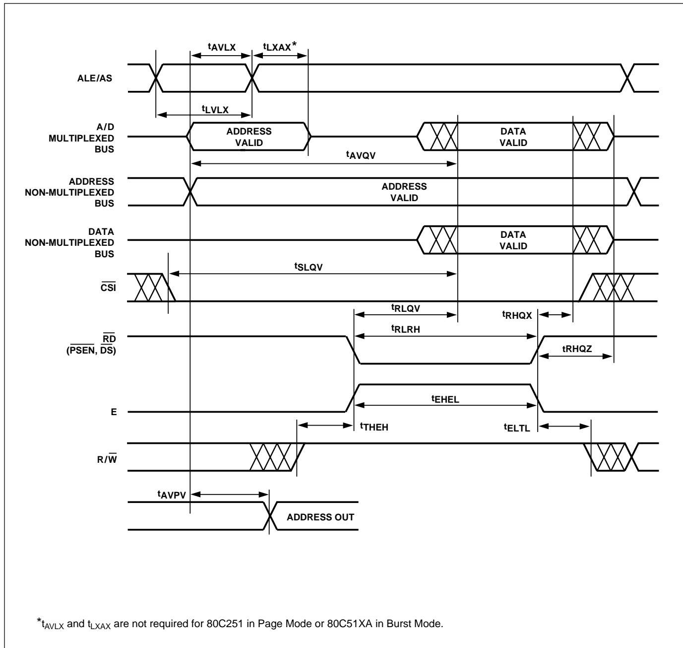
Figure 35. Read Timing
