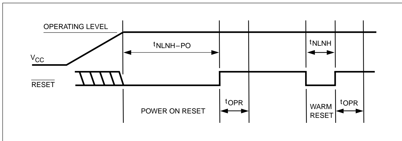
Figure 46. Reset Timing
