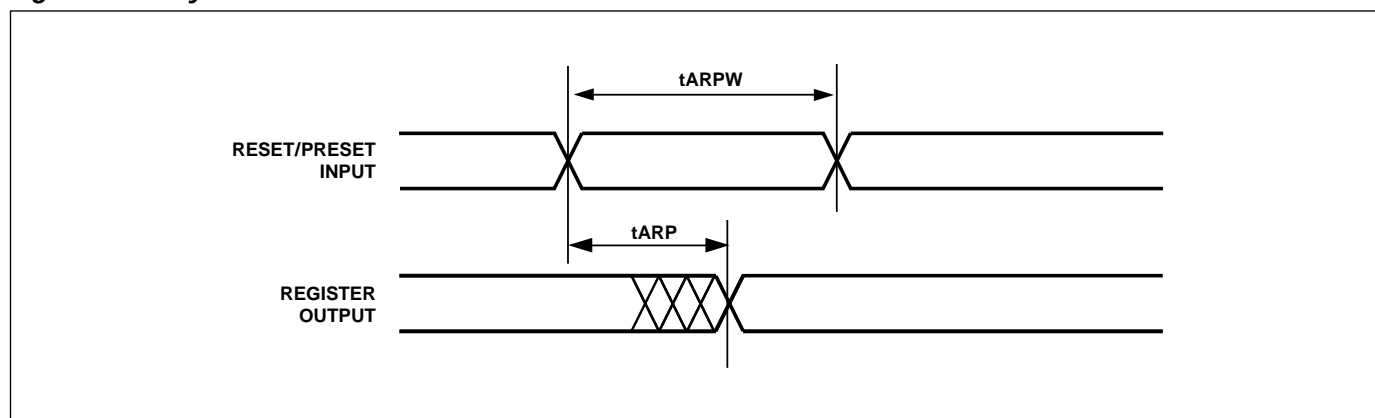
Figure 44. Asynchronous Reset/Preset
