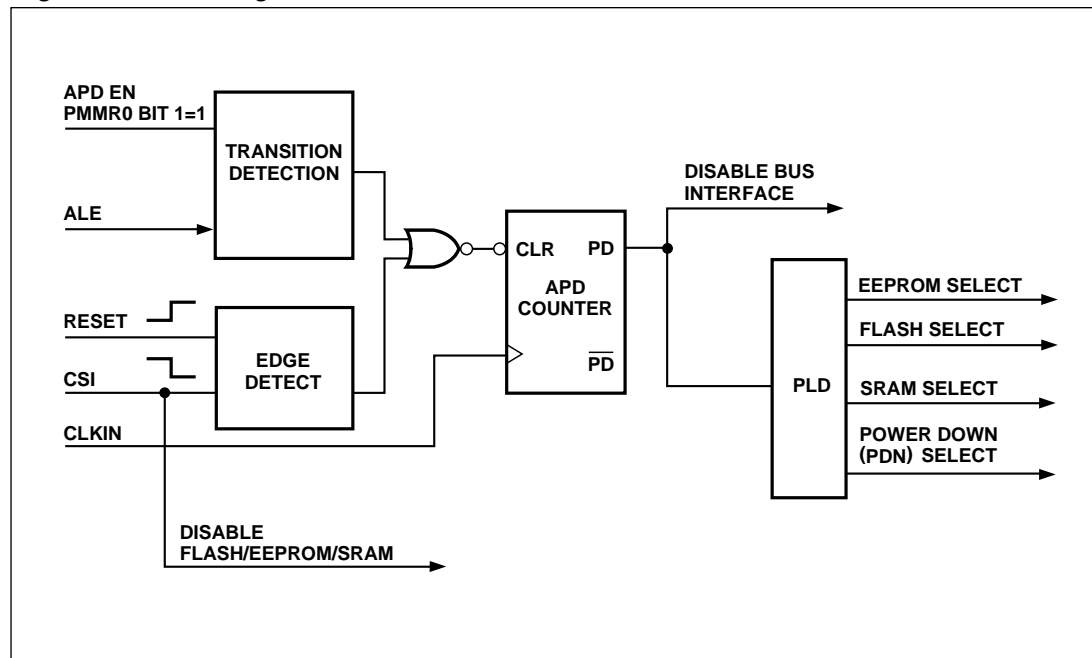
Figure 31. APD Logic Block
