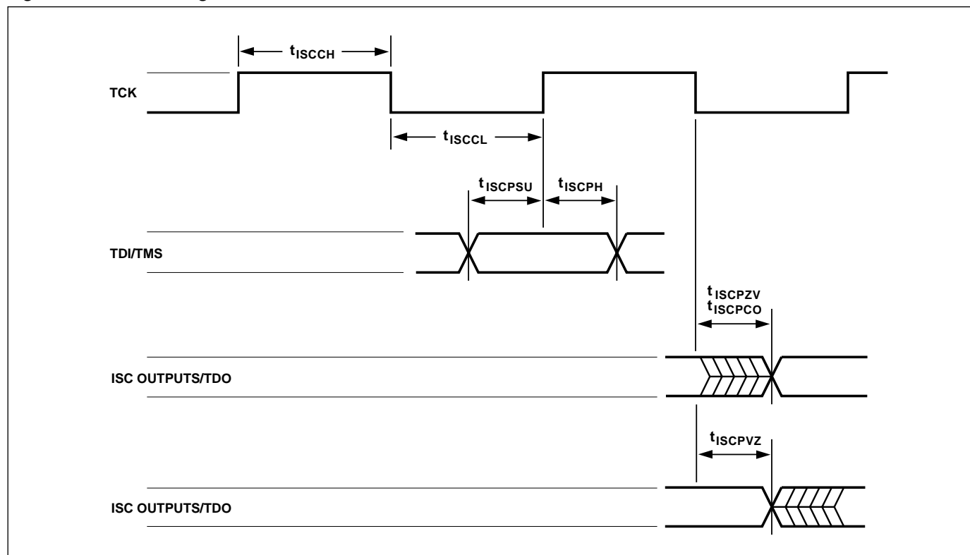
Figure 45. ISC Timing
