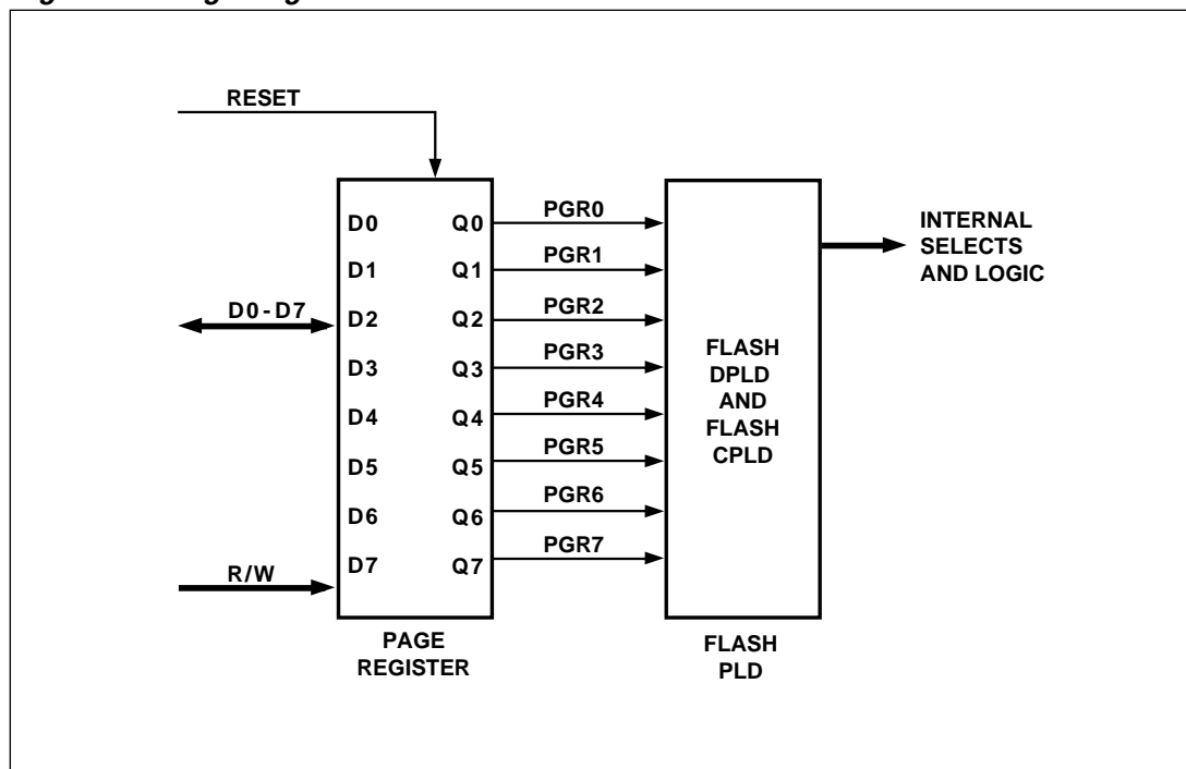
Figure 11. Page Register
