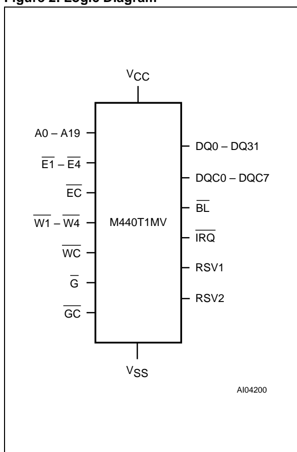
Figure 2. Logic Diagram
