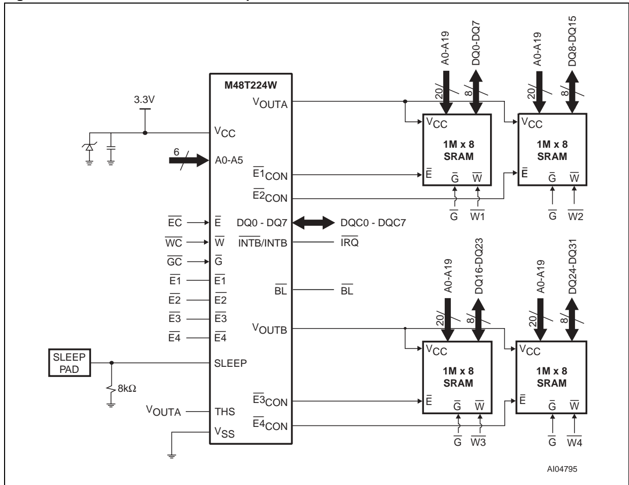
Figure 4. M440T1MV Hardware Hookup
