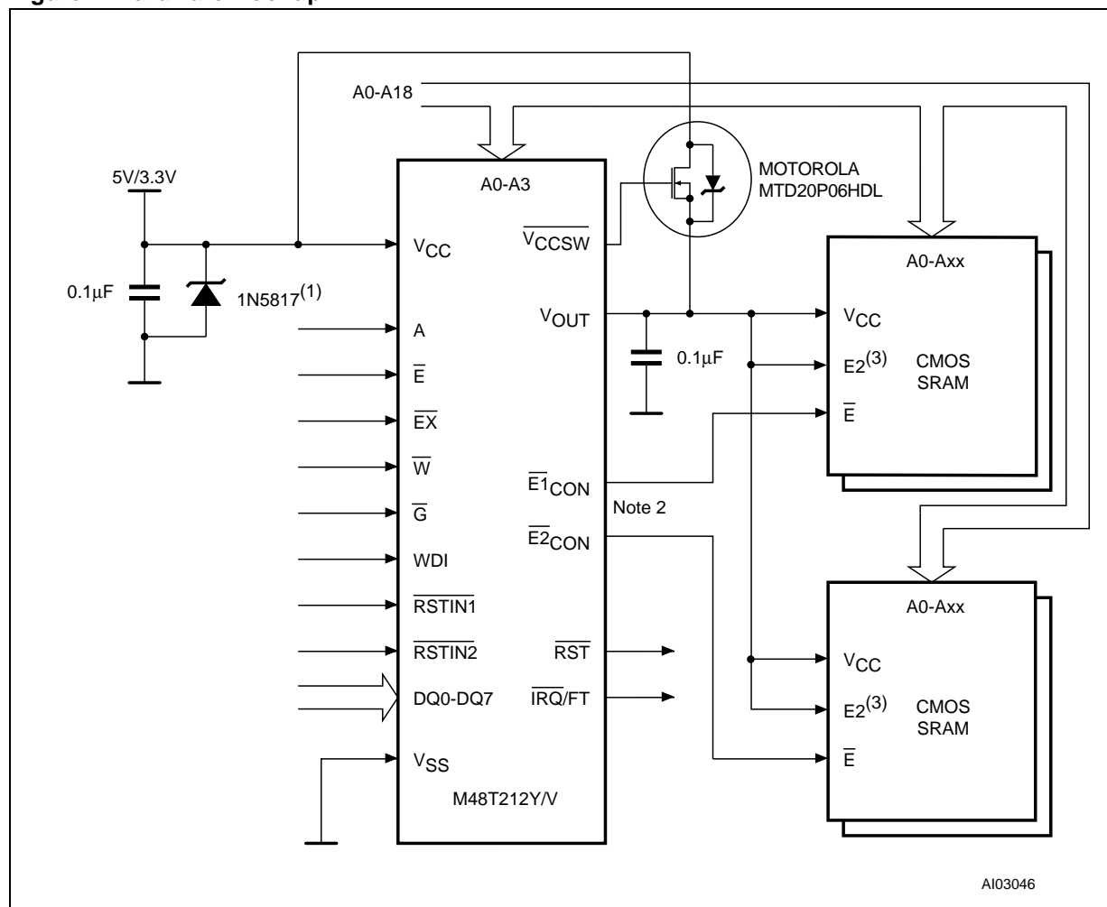
Figure 4. Hardware Hookup
