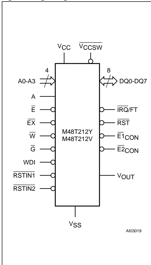
Figure 2. Logic Diagram
