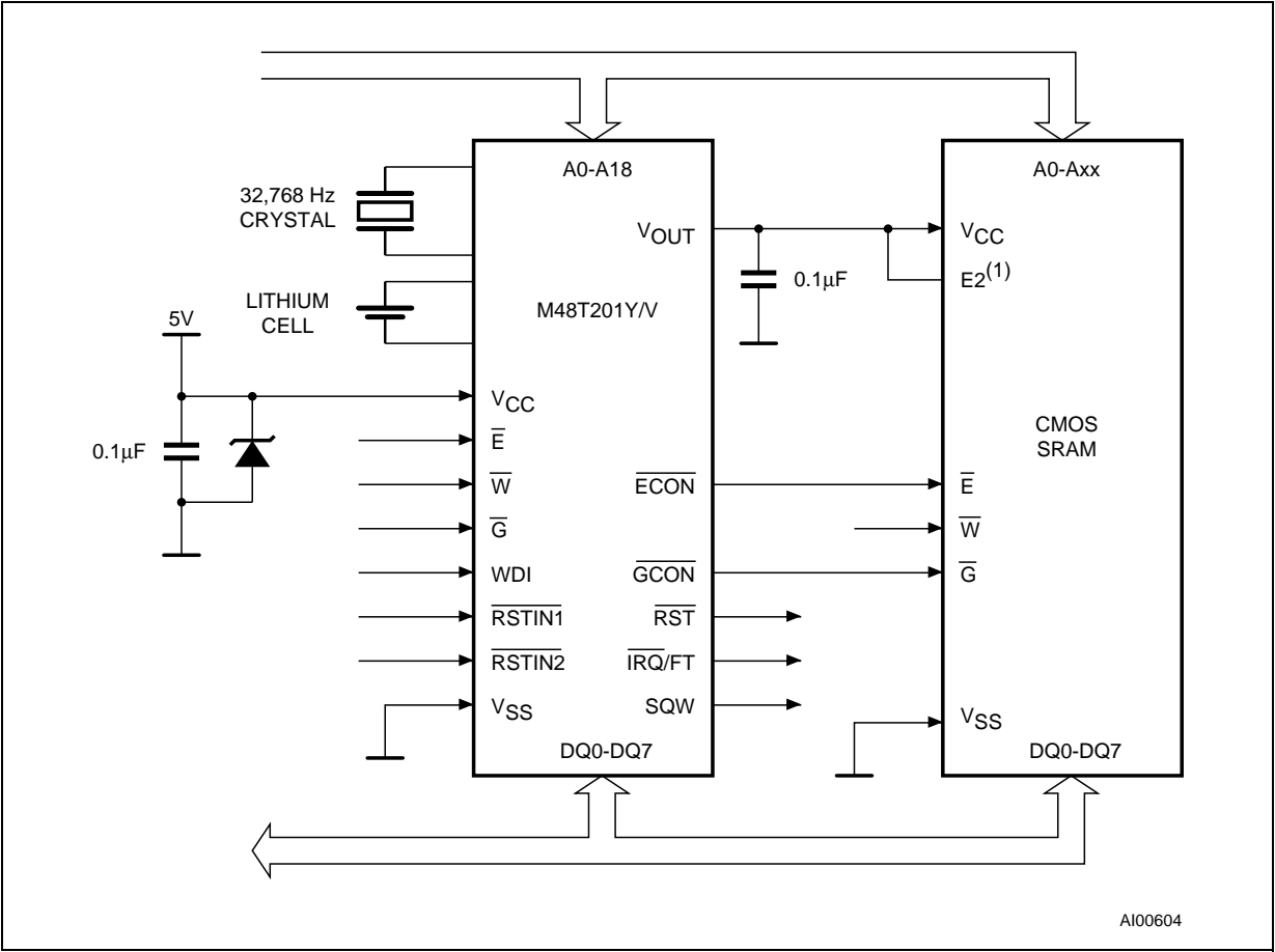
Figure 4. Hardware Hookup
