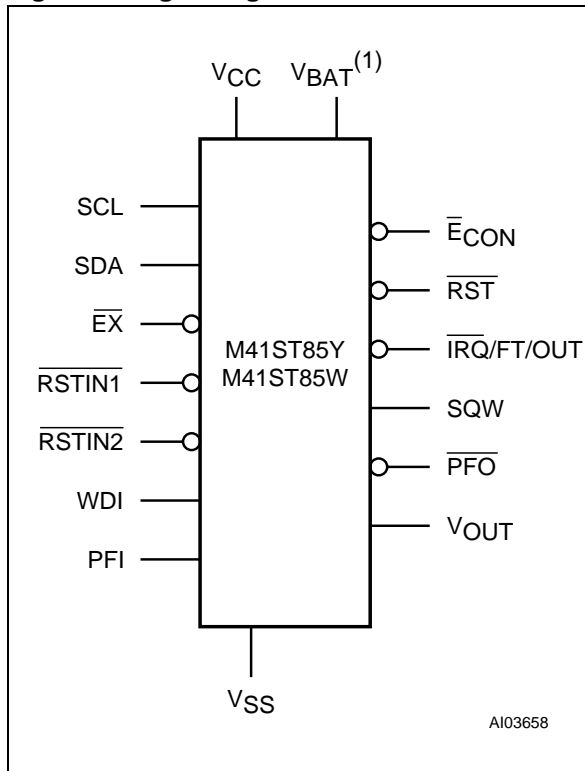
Figure 3. Logic Diagram
