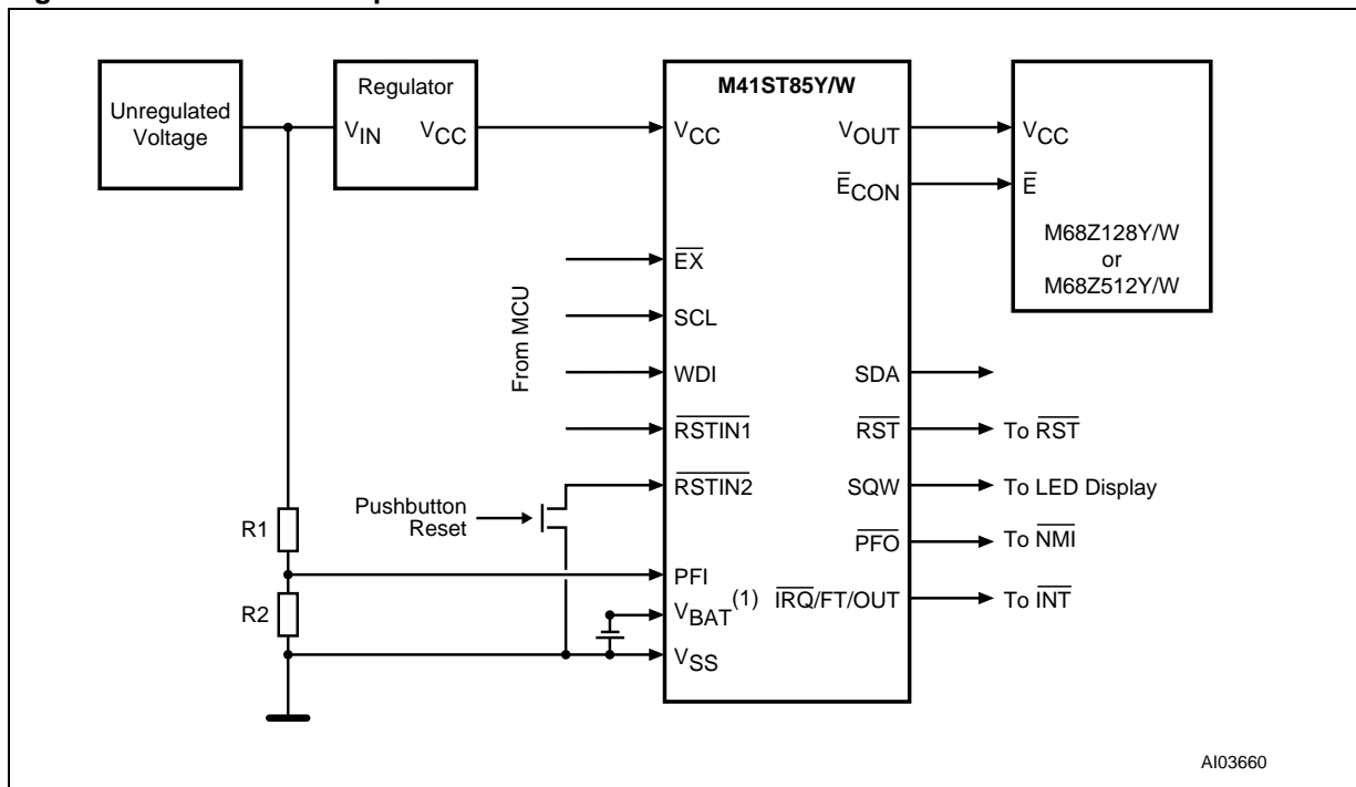
Figure 7. Hardware Hookup
