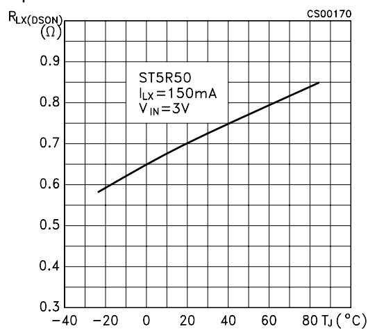
Figure 22 : Internal Switch R_{\text{DS(on)}} vs Temperature
