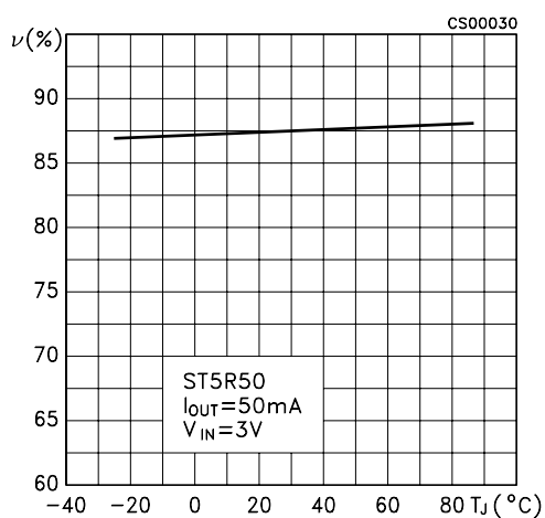
Figure 5 : Efficiency vs Temperature
