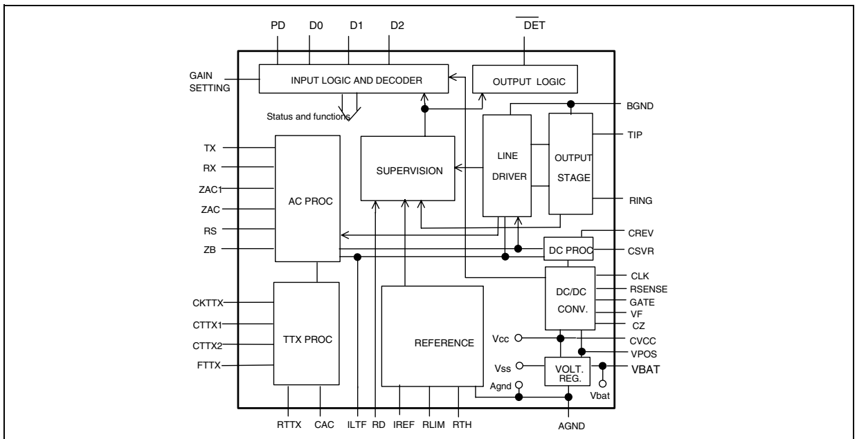
Figure 2. Block Diagram
