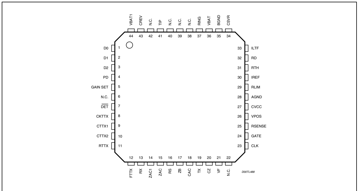
Figure 3. Pin Connection
