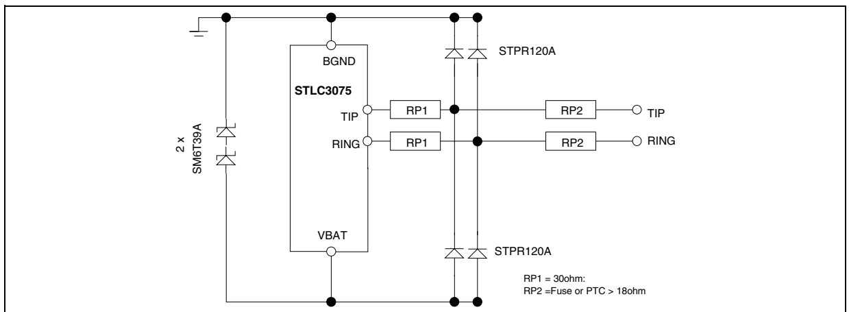
Figure 22. Simplified configuration for indoor overvoltage protection
