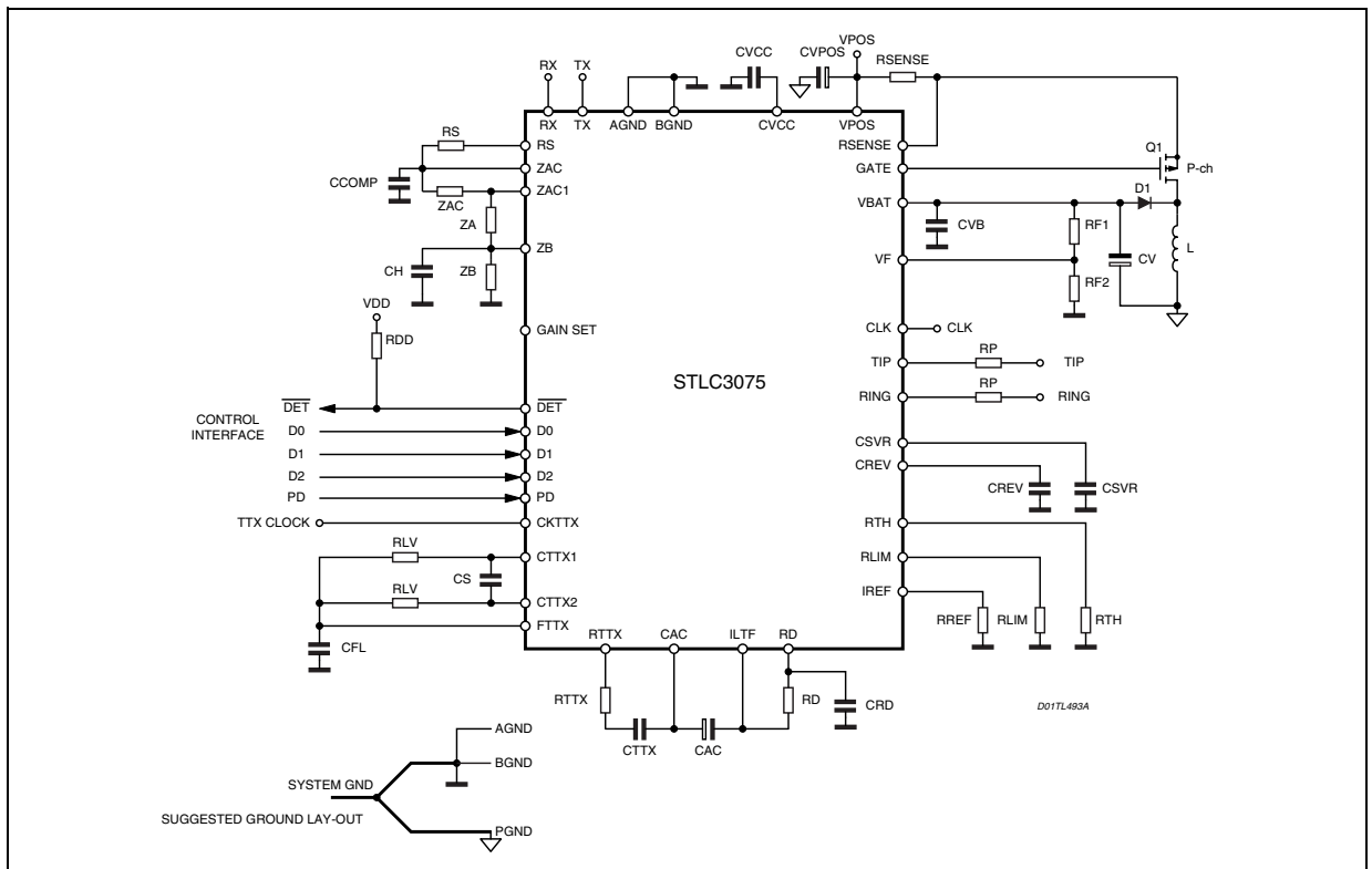
Figure 11. Application Diagram with P-Channel.
