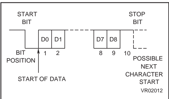
Figure 37. Character Format
