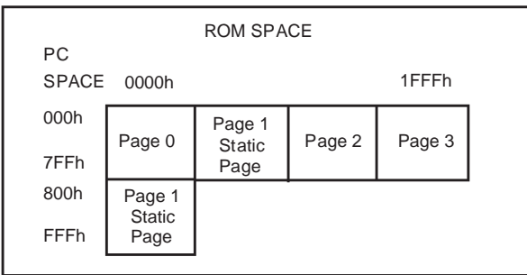
Figure 4. 8Kbytes Program Space Addressing
