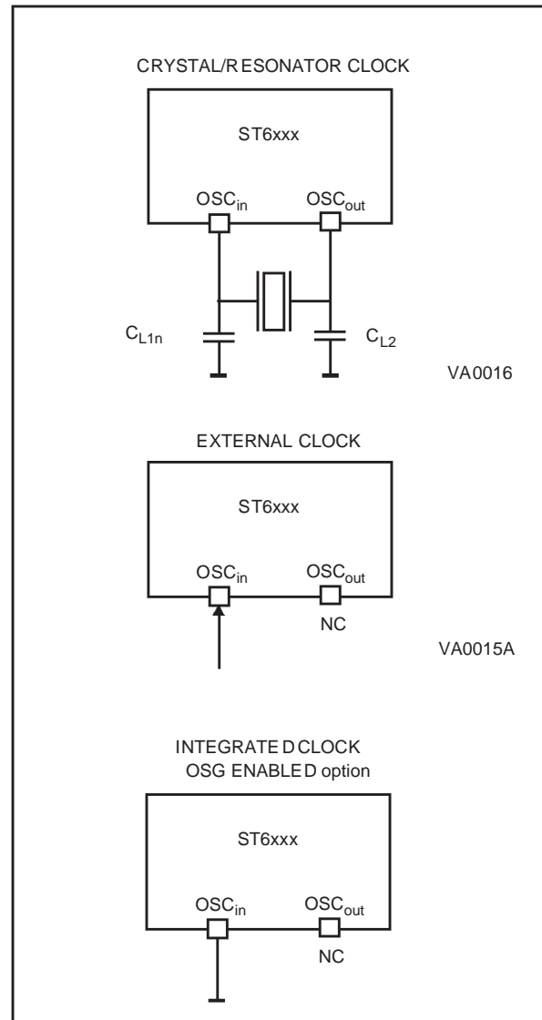
Figure 9. Oscillator Configurations
