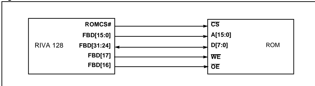
Figure 55. ROM interface
